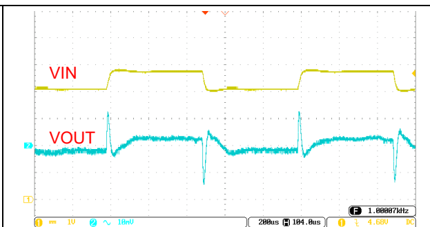
图 2 Line Transient ( V_{IN} =from 4.3V to 5V to 4.3V, I_{OUT} =300mA)
