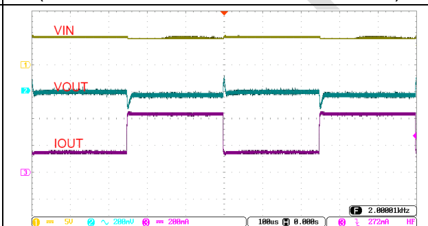
图 4 Load Transient ( V_{IN} =5.3V, I_{OUT} =150mA-300mA-150mA)
